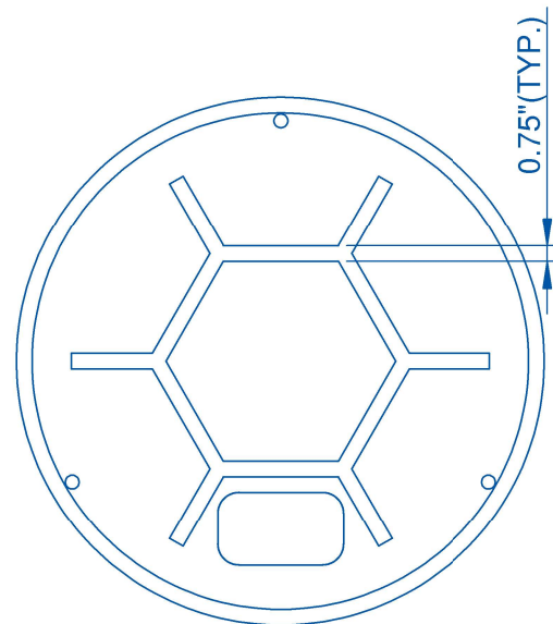
3/8" x 3/8" NEOPRENE GASKET
